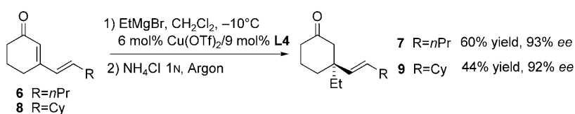
Scheme 4. Enantioselective 1,4-conjugate addition to other substrates. Cy = cyclohexyl.
