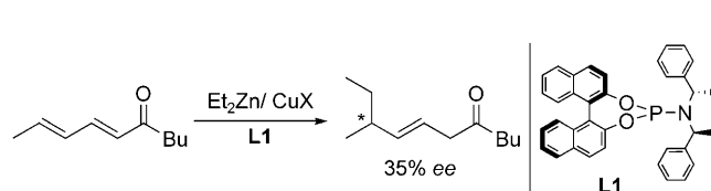
Scheme 1. 1,6 addition of diethyl zinc.
